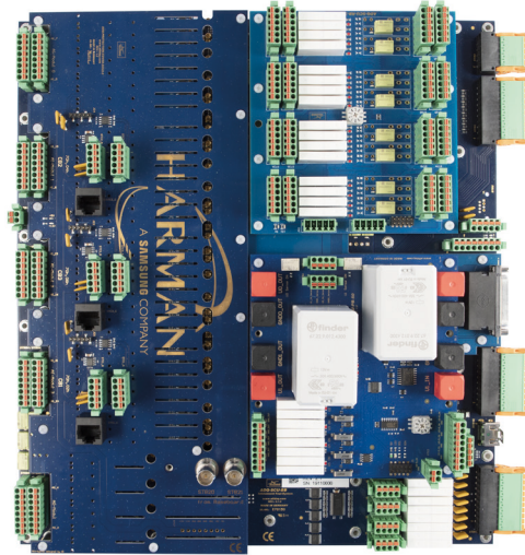
Abb. 2: Baseboard ADQ-SCU-BB
