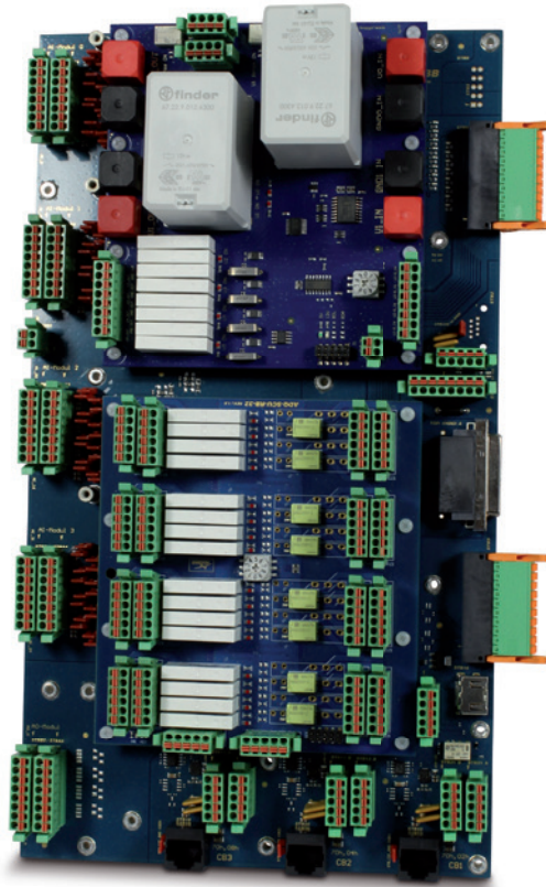
Abb. 2: Baseboard ADQ-SCU-LC-BB
