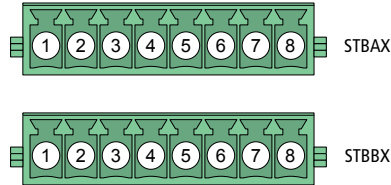
Figure 11: 8-pol. Würth-Steckverbinder
