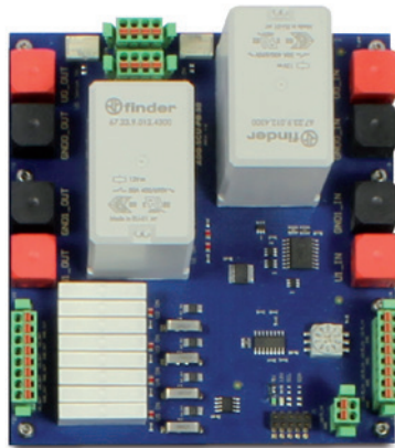
Abb. 3: Powerboard ADQ-SCU-LC-PB-50
