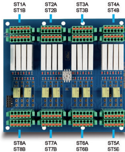
Abb. 4: Relaisboard ADQ-SCU-LC-RB-16/8
