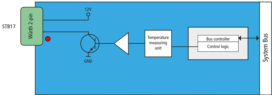
Figure 12: Fan control block diagram
