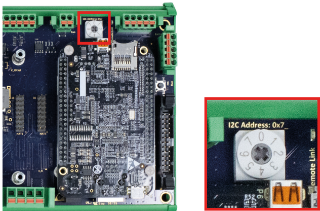
Figure 15: Rotary switch
