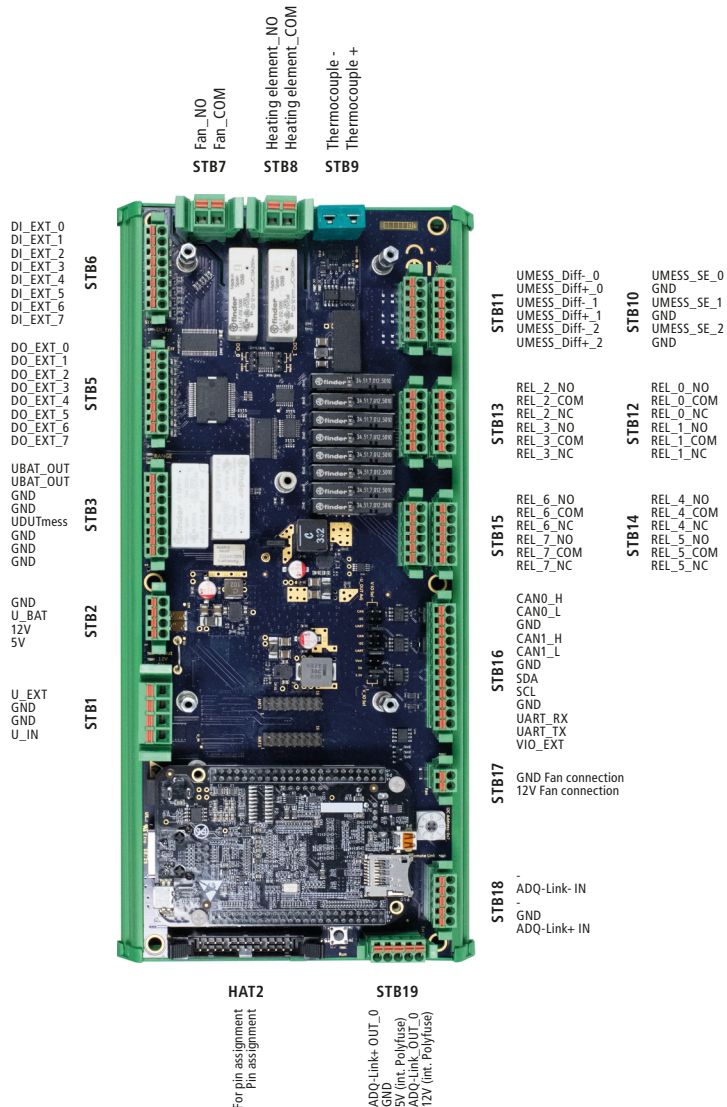
Figure 18: ADQ-CDI-BB with connector position/assignment
