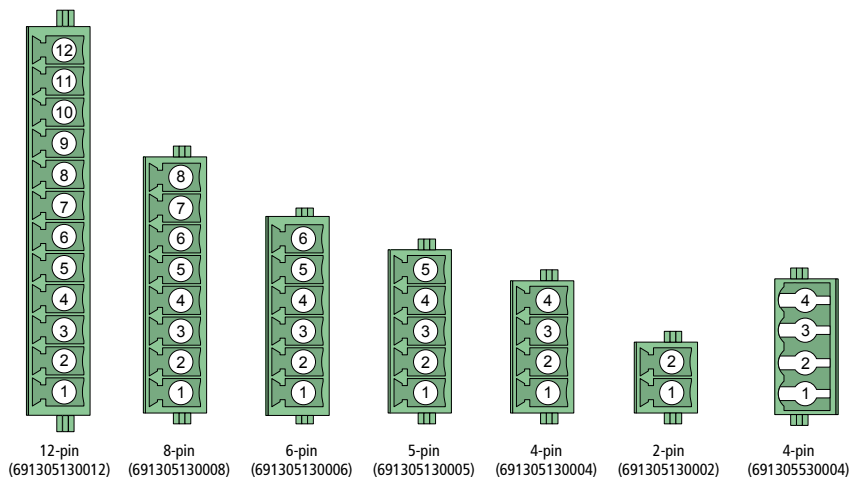
Figure 19: Würth baseboard Typee WR-TBL 3051 (top view)
