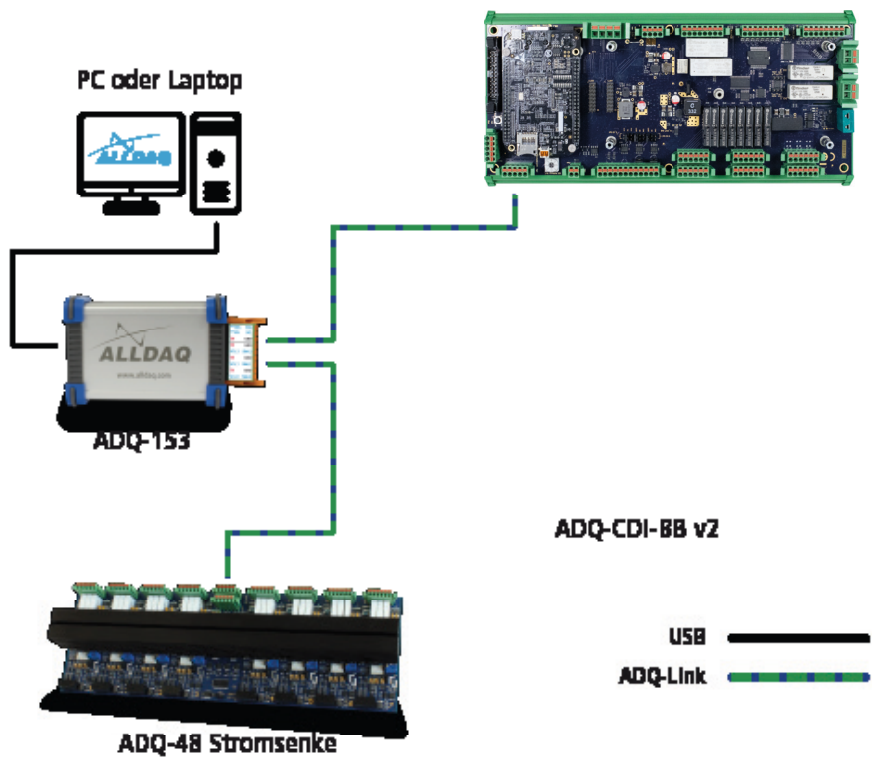
Figure 16: ADQ-153 as control controller
