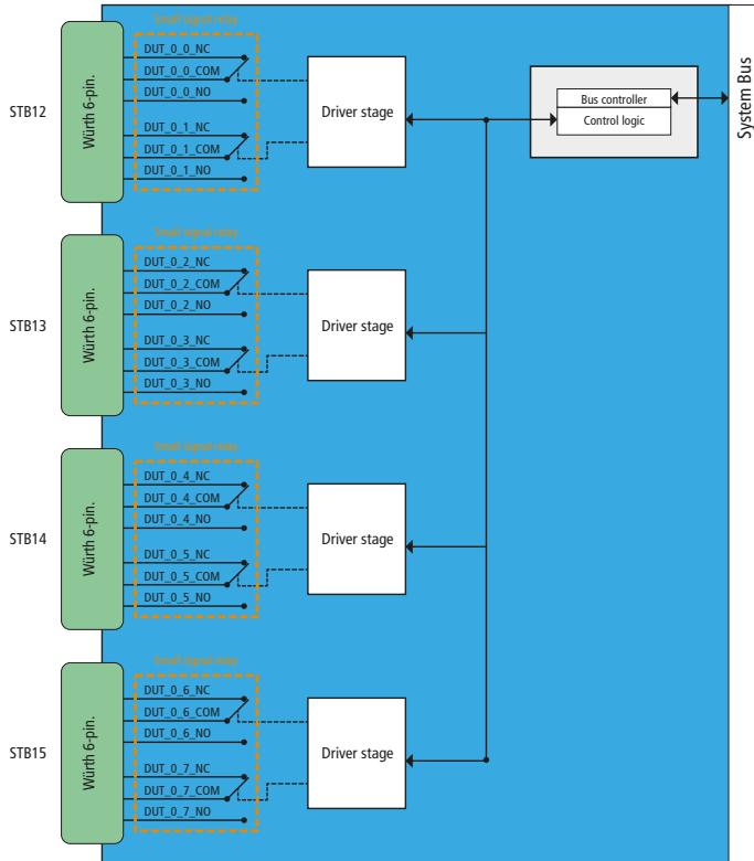
Figure 10: Relay block diagram
