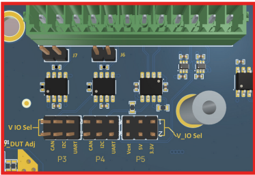
Figure 6: Jumper CAN/UART/I2C
