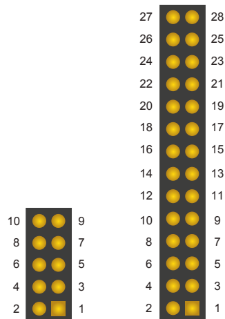
Figure 21: Male connector, 2.54mm (top view)
