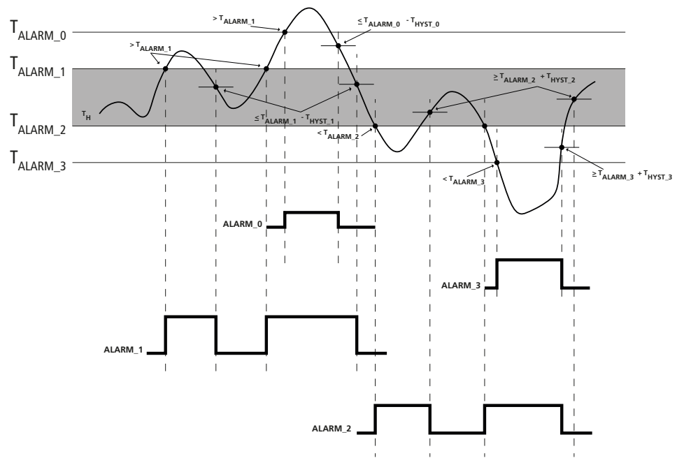
Figure 9: Alarm thresholds
