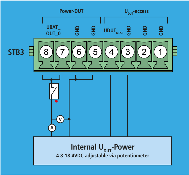
Figure 7: Block diagram of power measurement channels
