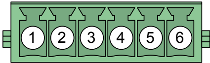
Figure 36: Würth 691305530006
