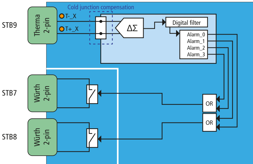
Figure 8: Block diagram of temperature measuring channel incl. alarm relay
