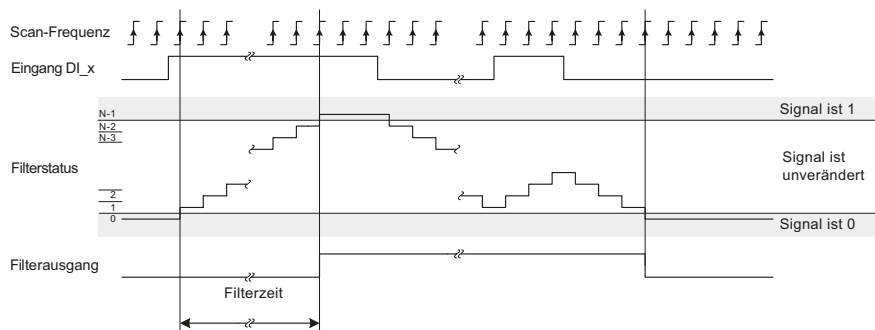
Figure 2: Digital input filter
