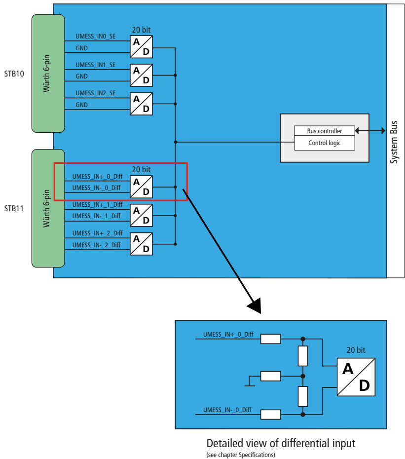
Figure 11: Block diagram of analog inputs
