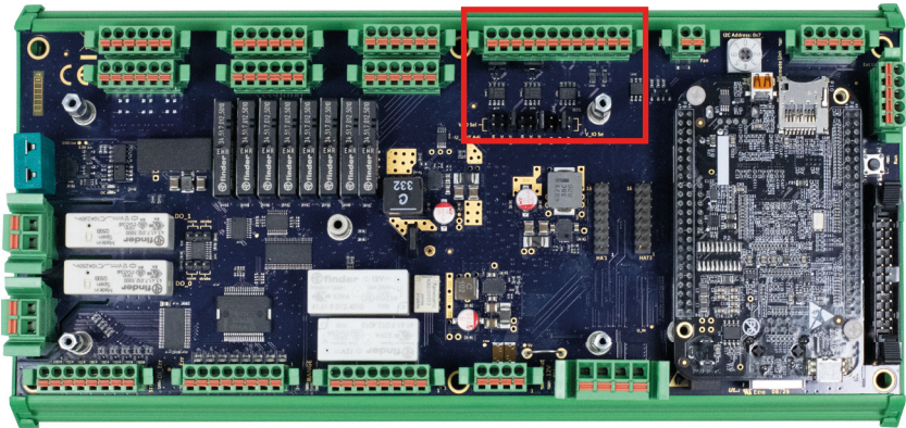
Figure 6: Jumper CAN/UART/I2C
