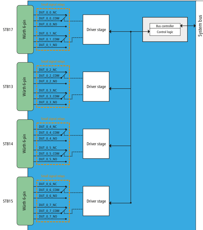
Figure 10: Block diagram relays
