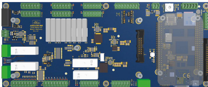
Figure 16: ADQ-CDI-BB with Beagle Bone Black single board computer
