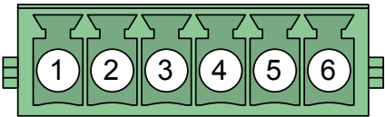
Figure 31: Würth 691305530006
