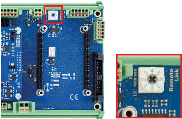
Abb. 14: Rotary switch
