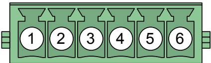
Figure 35: Würth 691305530006
