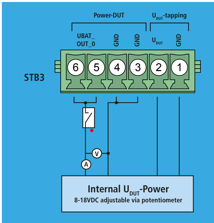
Figure 7: Block diagram power measurement channels
