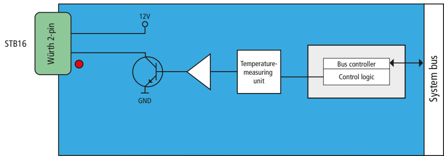
Figure 12: Block diagram fan control
