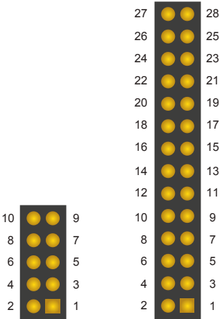
Figure 20: Pin connector, 2.54mm (top view)
