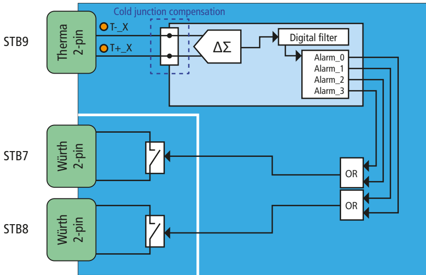
Figure 8: Block diagram temperature measuring channel incl. alarm relay
