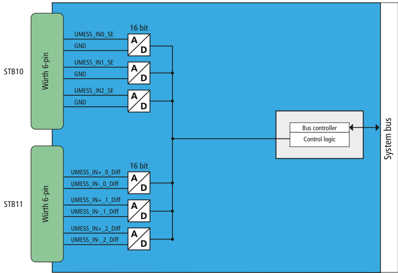
Figure 11: Block diagram analog inputs
